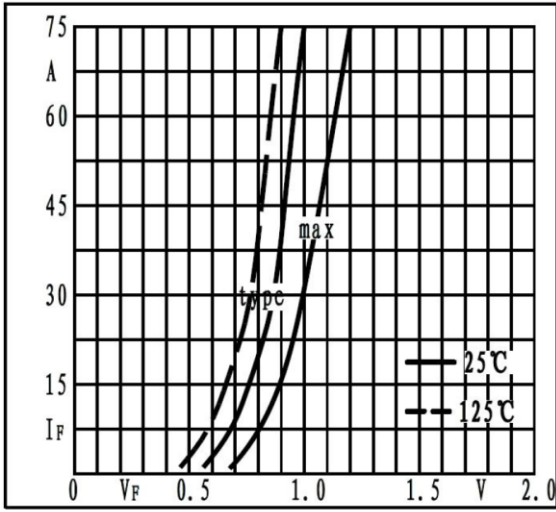
Fig1. Forward characteristics
