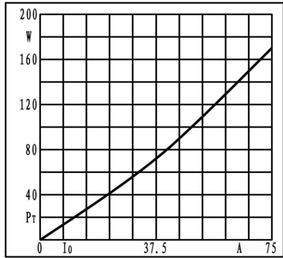
Fig2. Power dissipation
