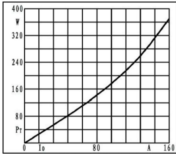
Fig2. Power dissipation
